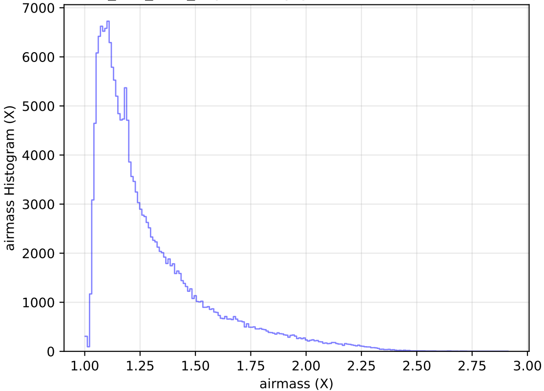
ddf_half_v3.4_10yrs All sky g band: airmass Histogram
