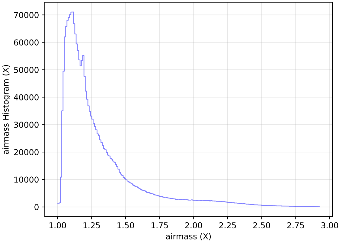
ddf_half_v3.4_10yrs All sky all bands: airmass Histogram
