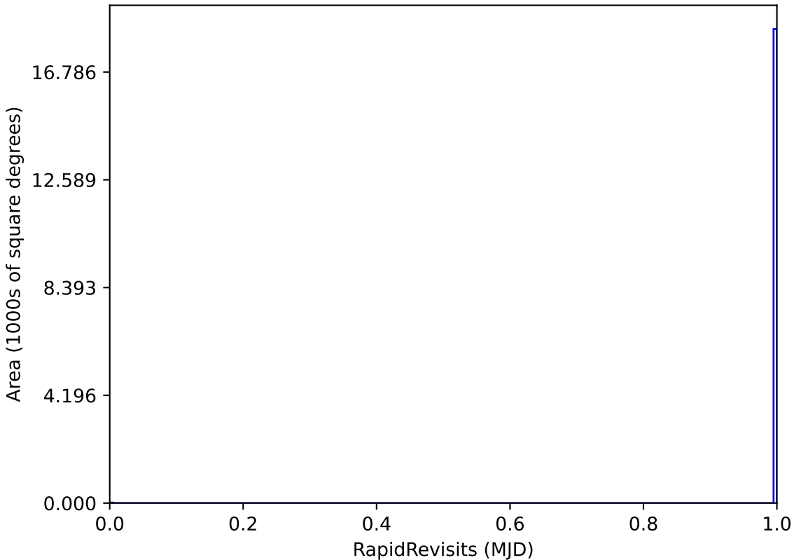
ddf_half_v3.4_10yrs WFD: RapidRevisits
