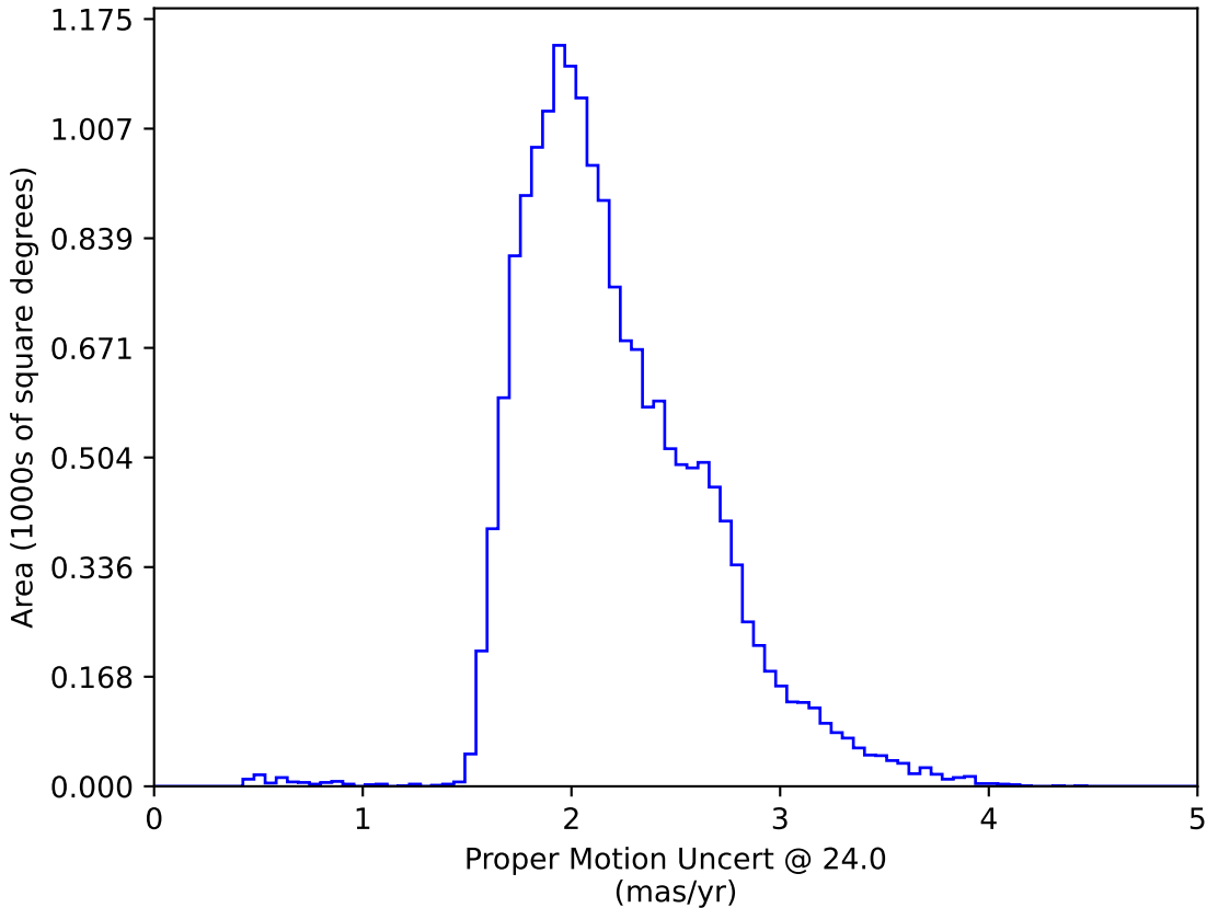
ddf_half_v3.4_10yrs WFD: Proper Motion Uncert @ 24.0
