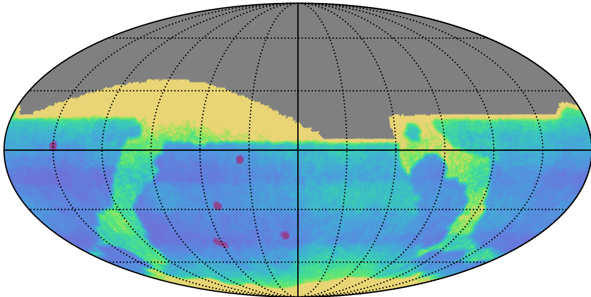
ddf_half_v3.4_10yrs All sky: Proper Motion Uncert @ 24.0
