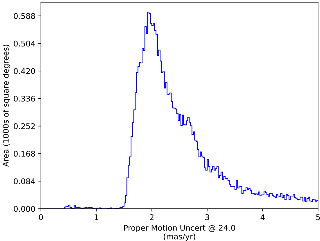
ddf_half_v3.4_10yrs All sky: Proper Motion Uncert @ 24.0
