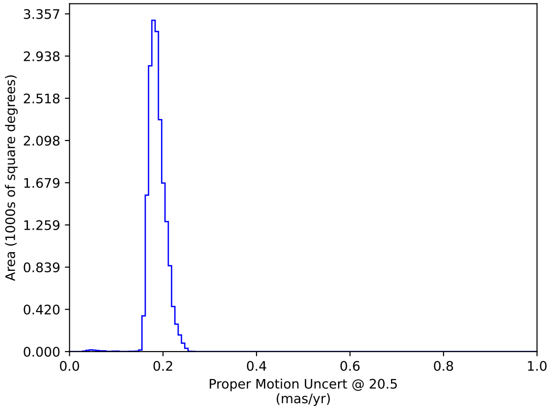
ddf_half_v3.4_10yrs WFD: Proper Motion Uncert @ 20.5
