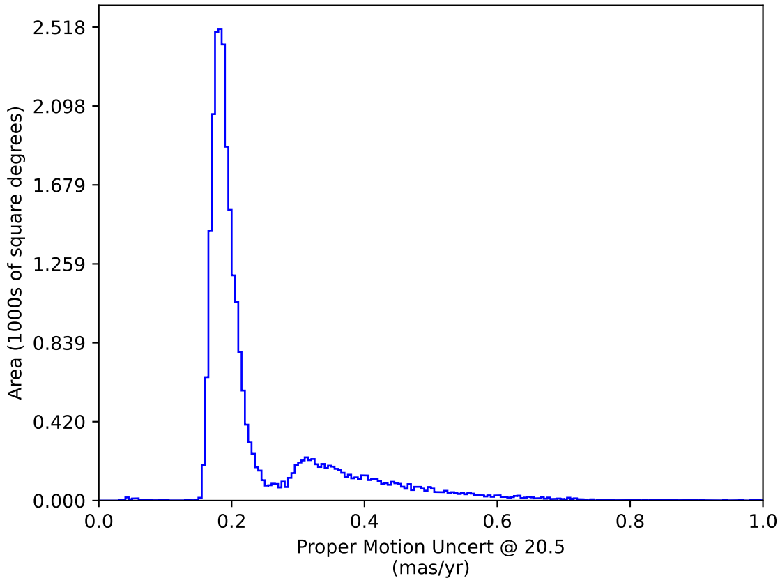
ddf_half_v3.4_10yrs All sky: Proper Motion Uncert @ 20.5
