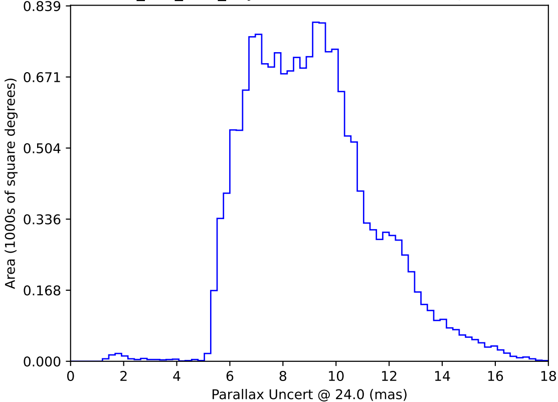
ddf_half_v3.4_10yrs WFD: Parallax Uncert @ 24.0
