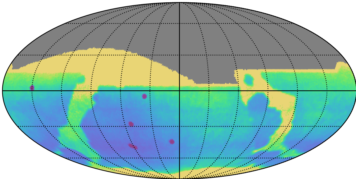
ddf_half_v3.4_10yrs All sky: Parallax Uncert @ 24.0
