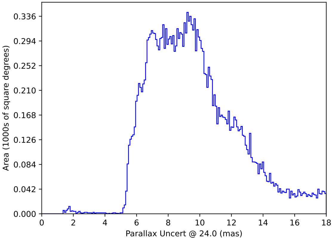
ddf_half_v3.4_10yrs All sky: Parallax Uncert @ 24.0
