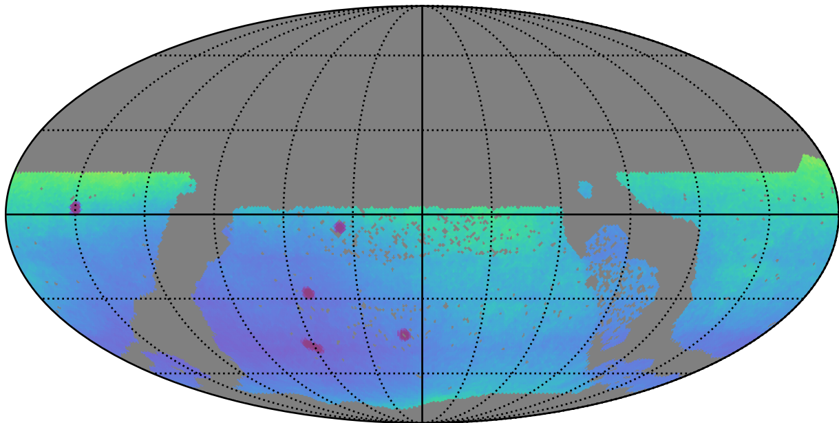
ddf_half_v3.4_10yrs WFD: Parallax Uncert @ 22.4
