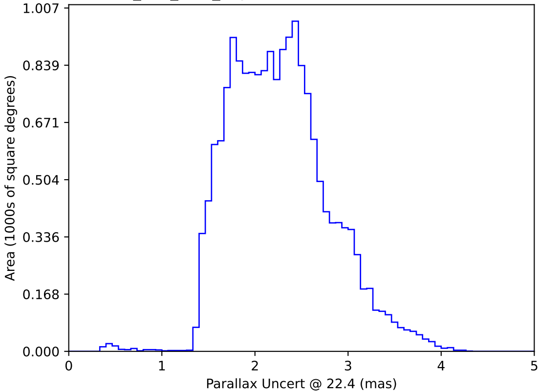
ddf_half_v3.4_10yrs WFD: Parallax Uncert @ 22.4
