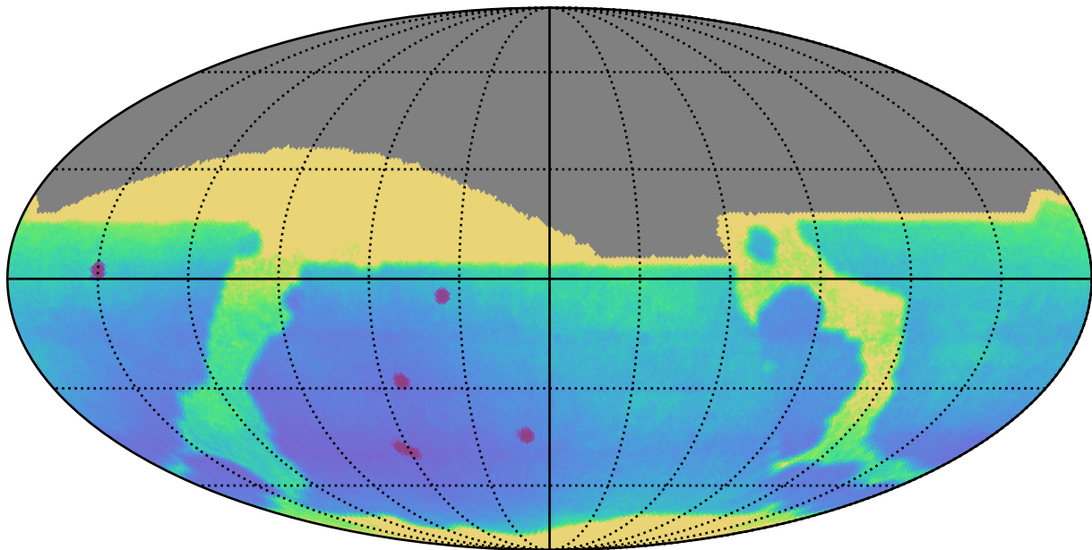
ddf_half_v3.4_10yrs All sky: Parallax Uncert @ 22.4
