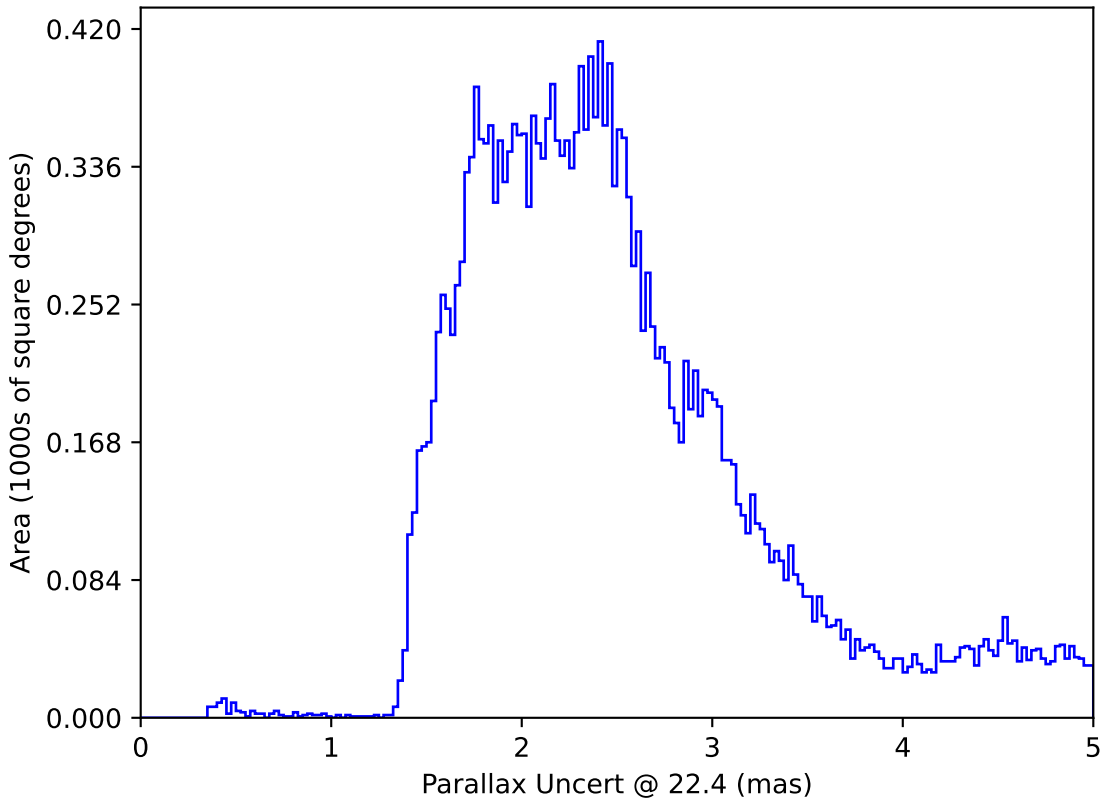
ddf_half_v3.4_10yrs All sky: Parallax Uncert @ 22.4
