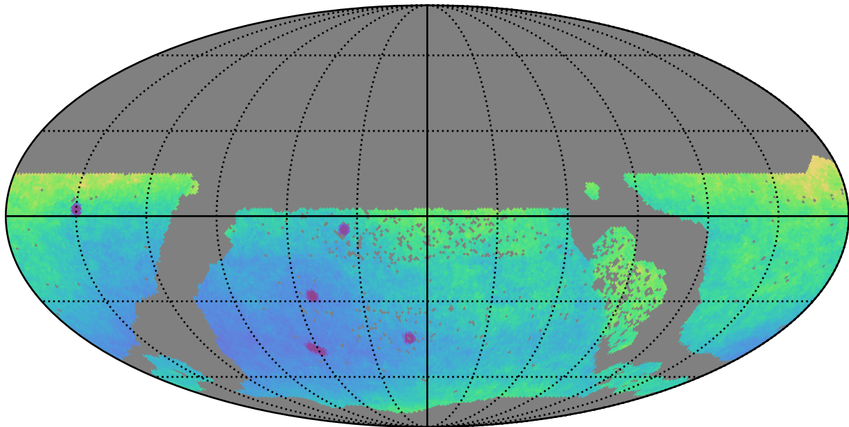
ddf_half_v3.4_10yrs WFD y band only: Parallax Uncert @ 21.3
