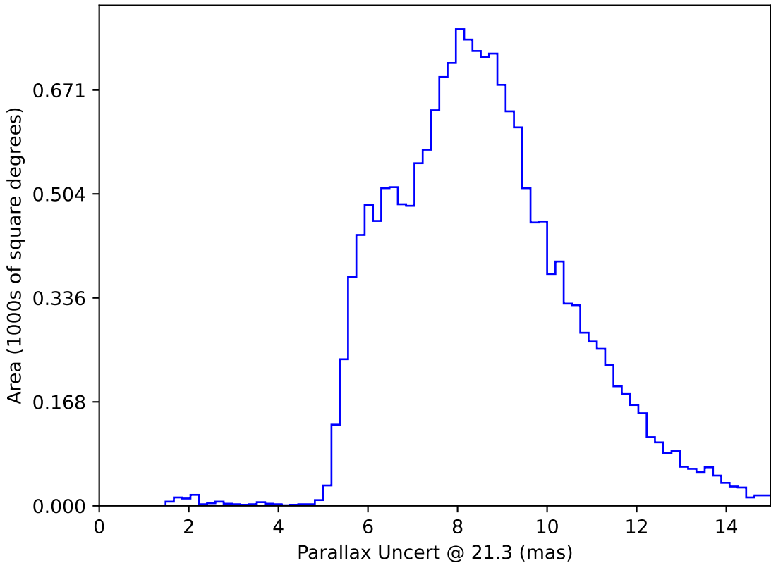
ddf_half_v3.4_10yrs WFD y band only: Parallax Uncert @ 21.3
