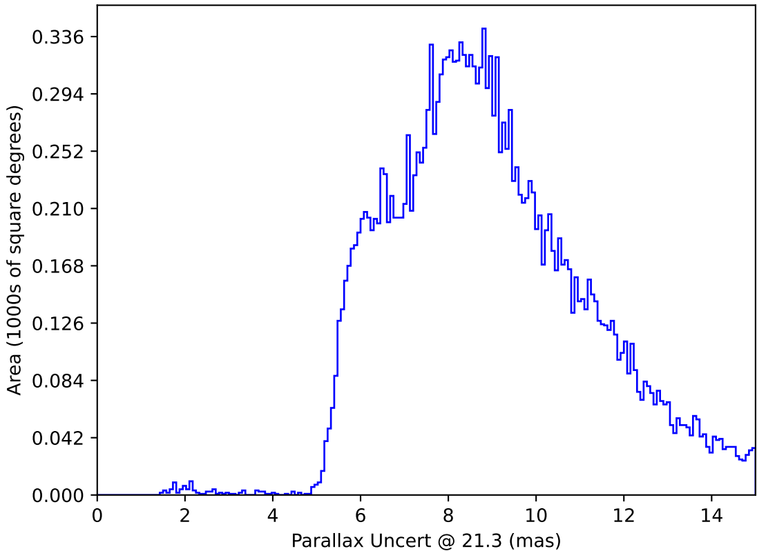
ddf_half_v3.4_10yrs All sky y band only: Parallax Uncert @ 21.3
