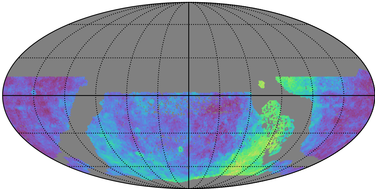
ddf_half_v3.4_10yrs WFD: Parallax Coverage @ 24.0
