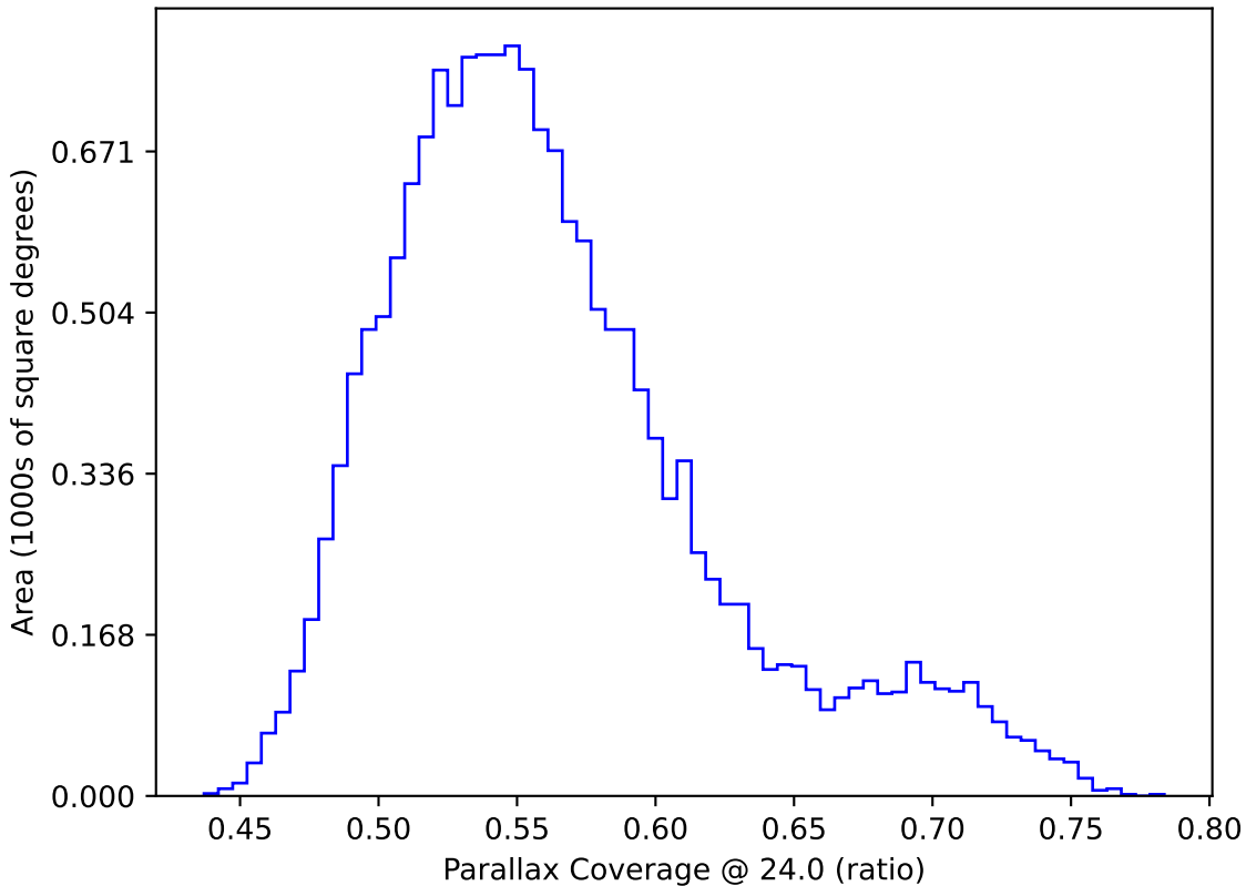
ddf_half_v3.4_10yrs WFD: Parallax Coverage @ 24.0
