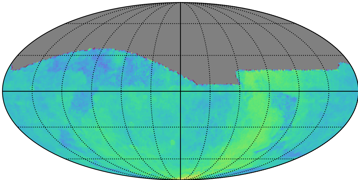
ddf_half_v3.4_10yrs All sky: Parallax Coverage @ 24.0
