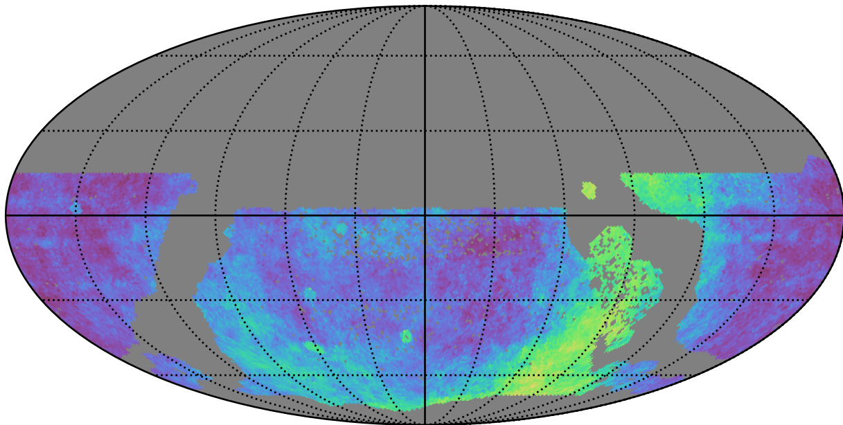
ddf_half_v3.4_10yrs WFD: Parallax Coverage @ 22.4
