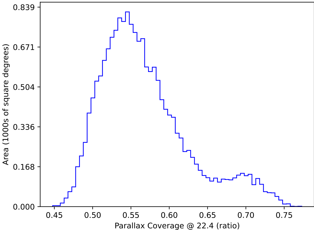
ddf_half_v3.4_10yrs WFD: Parallax Coverage @ 22.4
