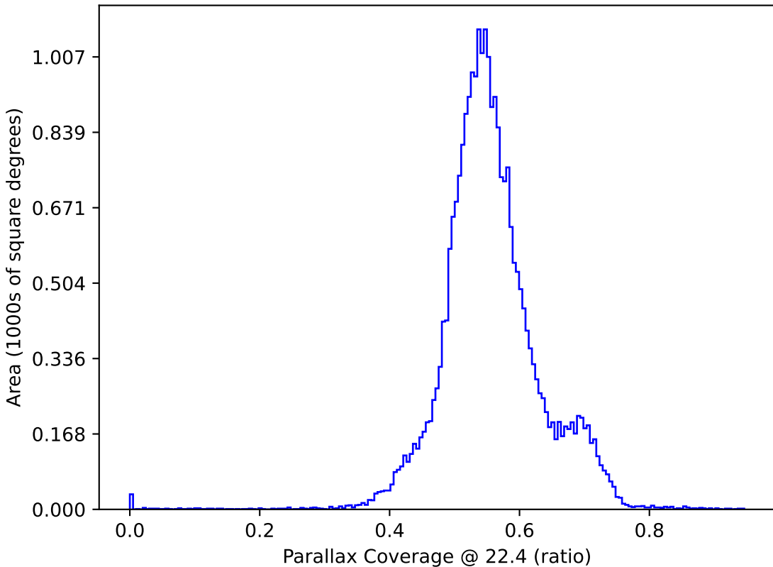
ddf_half_v3.4_10yrs All sky: Parallax Coverage @ 22.4
