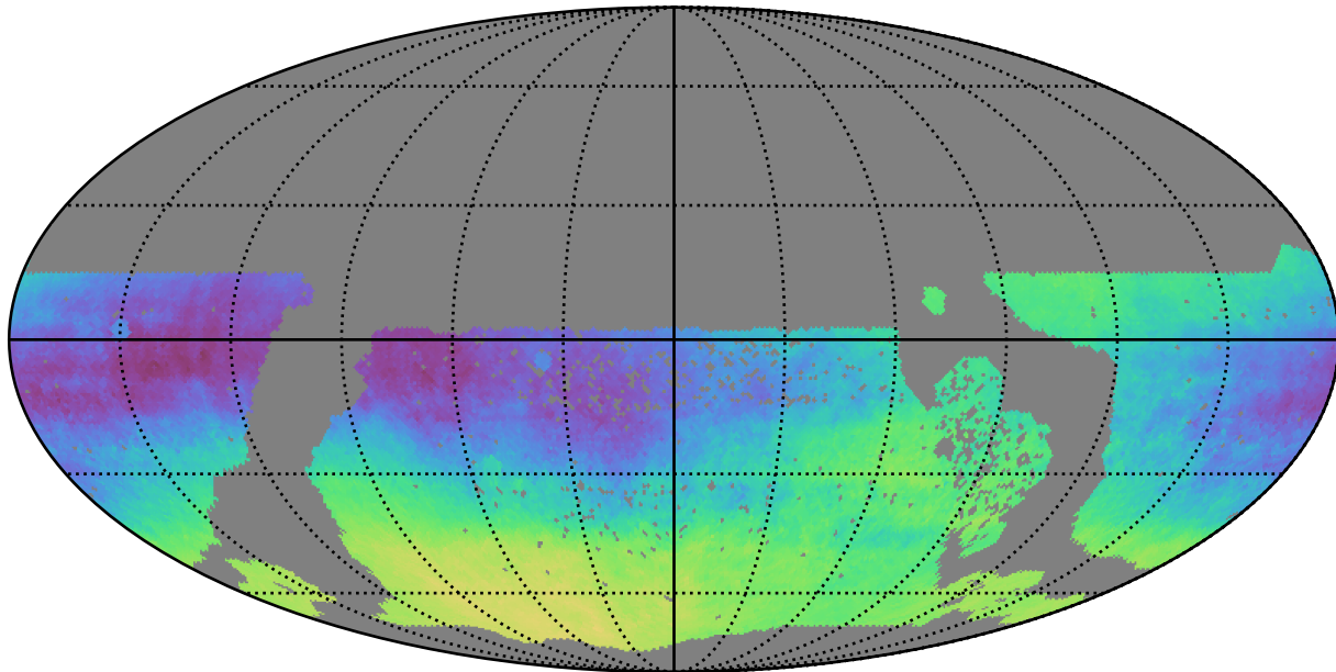
ddf_half_v3.4_10yrs WFD: Parallax-DCR degeneracy @ 24.0
