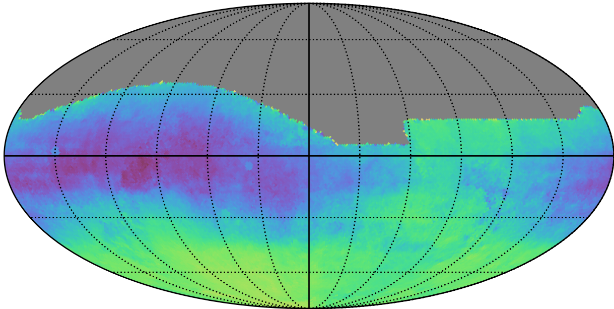
ddf_half_v3.4_10yrs All sky: Parallax-DCR degeneracy @ 24.0
