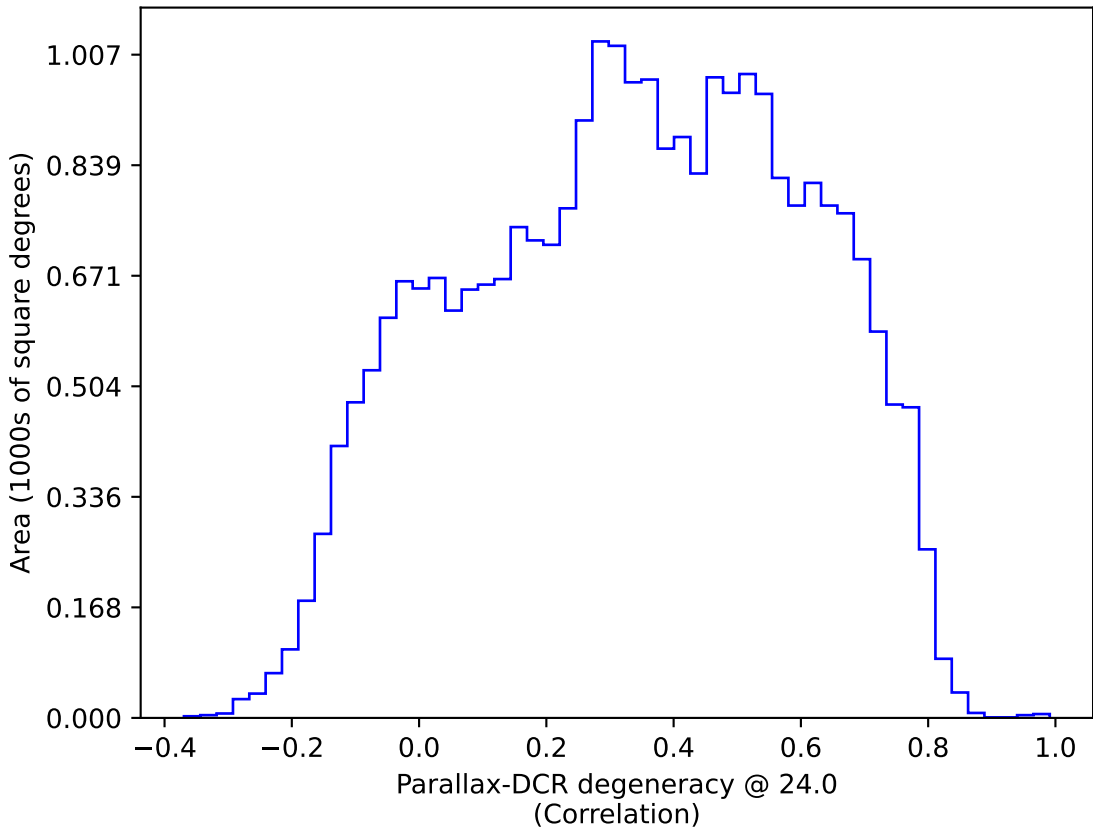
ddf_half_v3.4_10yrs All sky: Parallax-DCR degeneracy @ 24.0
