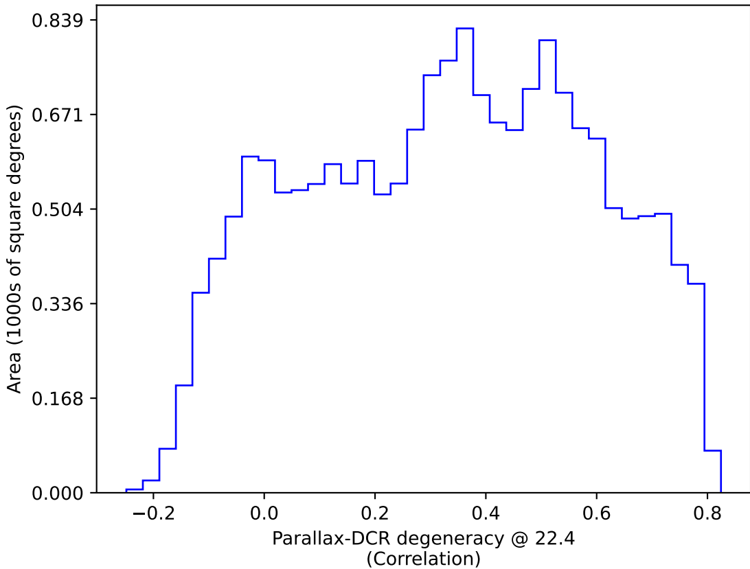
ddf_half_v3.4_10yrs WFD: Parallax-DCR degeneracy @ 22.4
