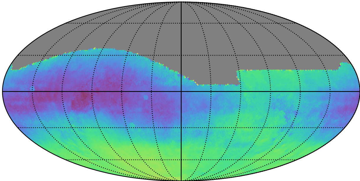
ddf_half_v3.4_10yrs All sky: Parallax-DCR degeneracy @ 22.4
