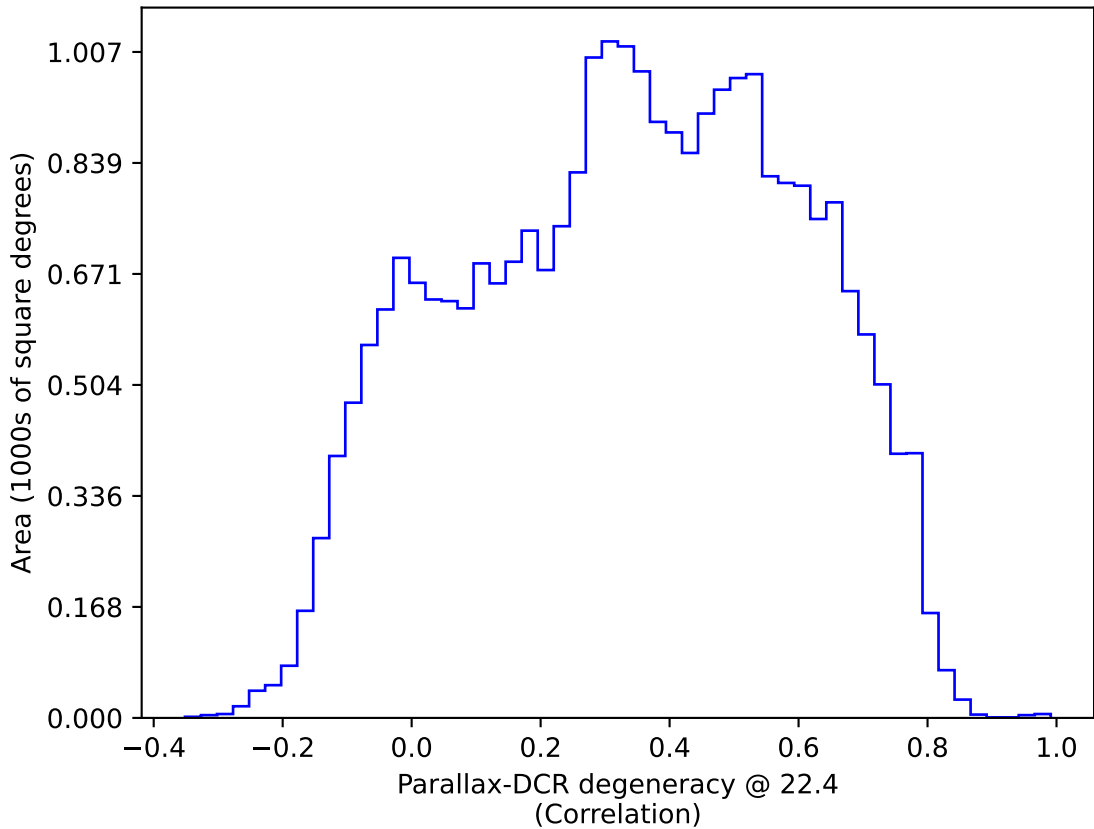
ddf_half_v3.4_10yrs All sky: Parallax-DCR degeneracy @ 22.4
