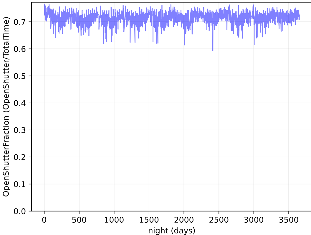
ddf_half_v3.4_10yrs Per night: OpenShutterFraction
