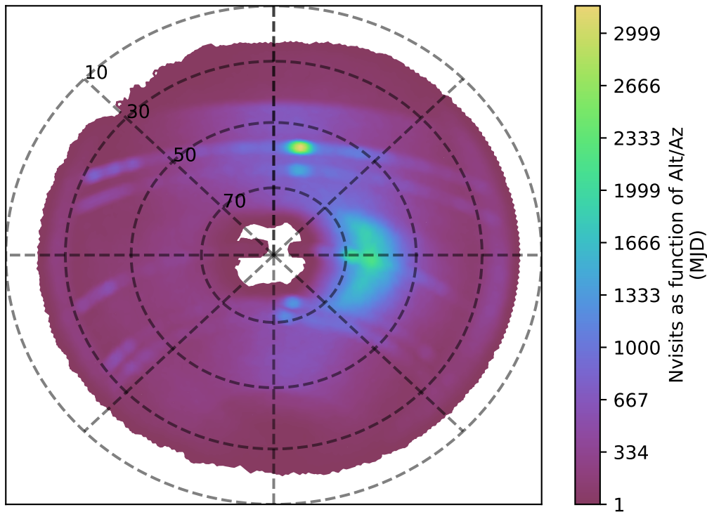
ddf_half_v3.4_10yrs z band: Nvisits as function of Alt/Az
