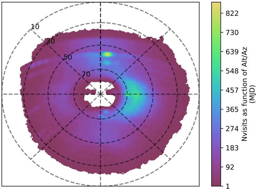
ddf_half_v3.4_10yrs u band: Nvisits as function of Alt/Az
