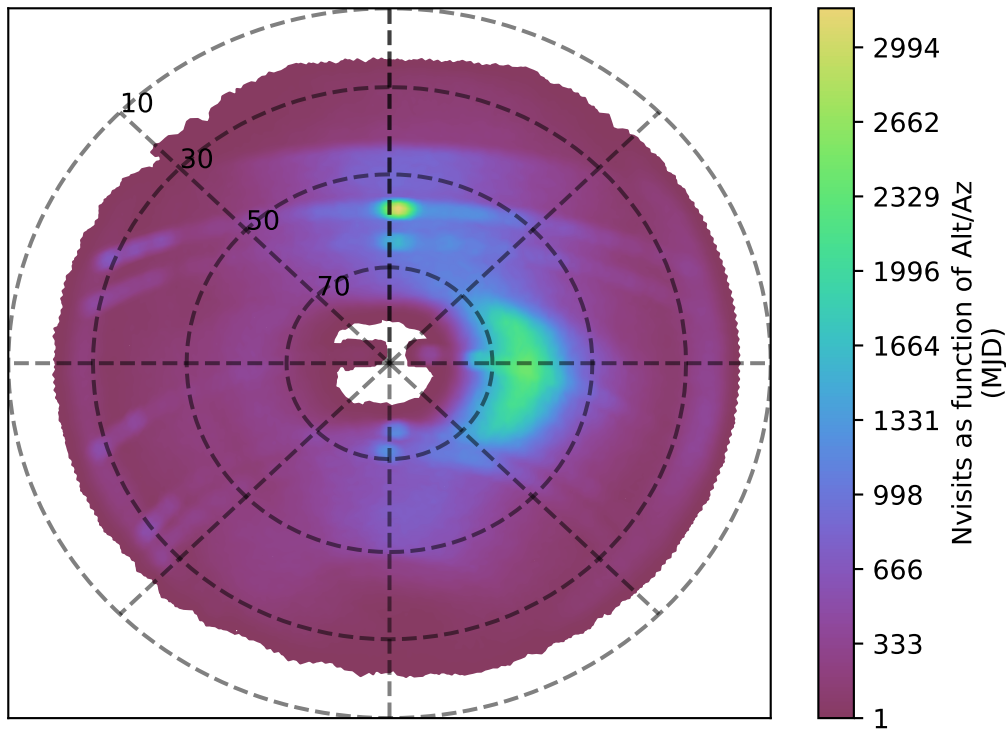
ddf_half_v3.4_10yrs i band: Nvisits as function of Alt/Az
