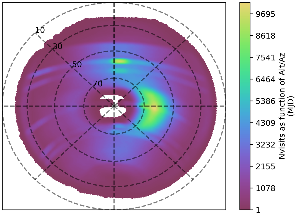
ddf_half_v3.4_10yrs all bands: Nvisits as function of Alt/Az
