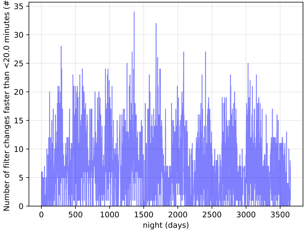
ddf_half_v3.4_10yrs Per Night: Number of filter changes faster than <20.0 minutes
