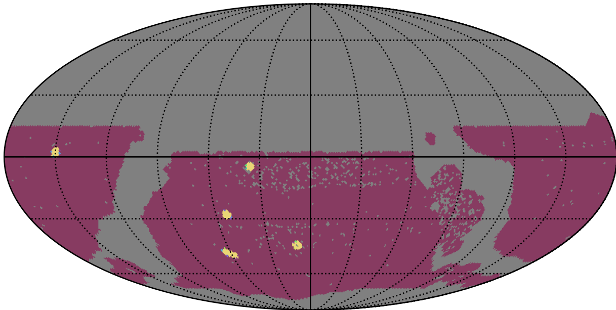
ddf_half_v3.4_10yrs WFD: NumberOfQuickRevisits
