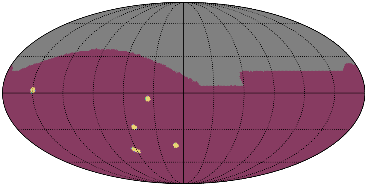
ddf_half_v3.4_10yrs All sky: NumberOfQuickRevisits
