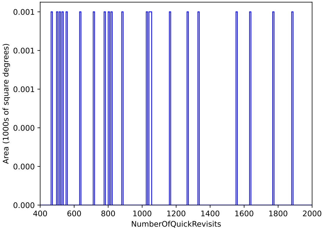
ddf_half_v3.4_10yrs All sky: NumberOfQuickRevisits
