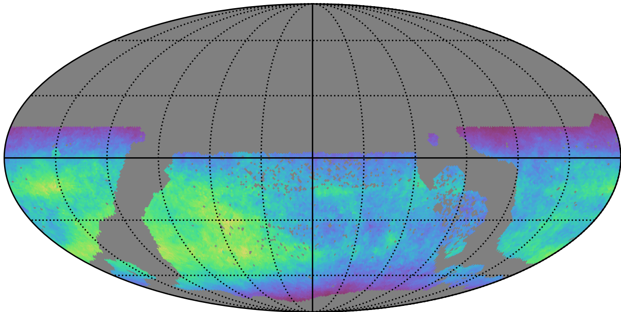
ddf_half_v3.4_10yrs WFD z band: Normalized Teff
