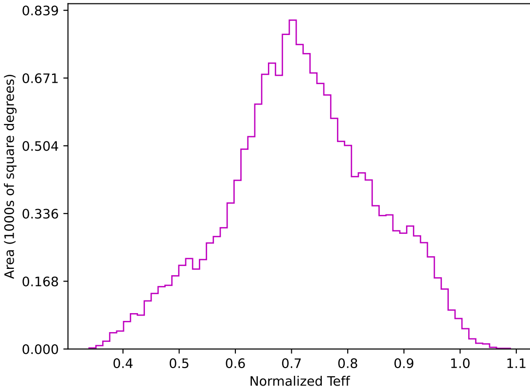
ddf_half_v3.4_10yrs WFD z band: Normalized Teff
