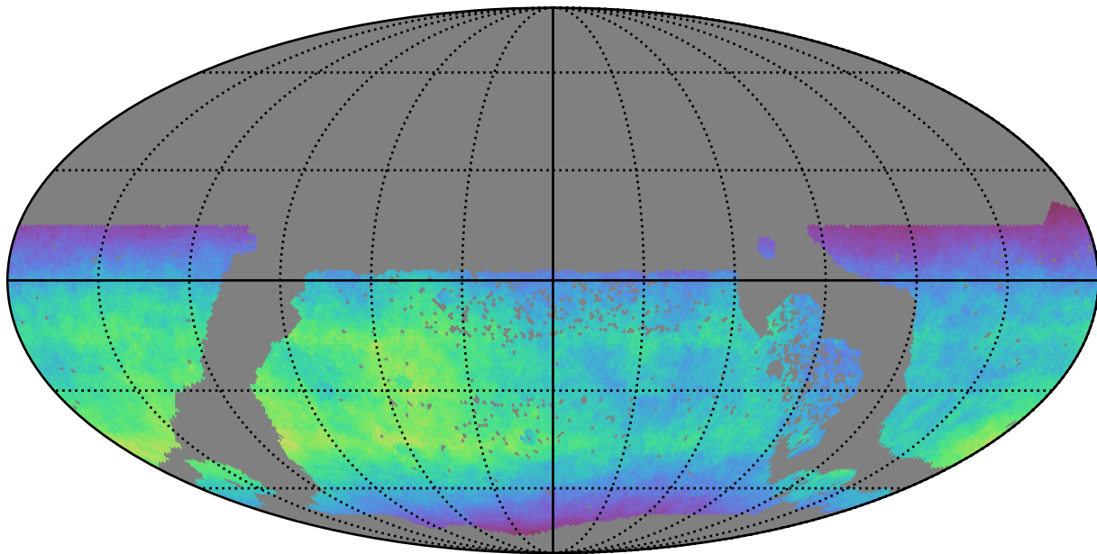
ddf_half_v3.4_10yrs WFD y band: Normalized Teff
