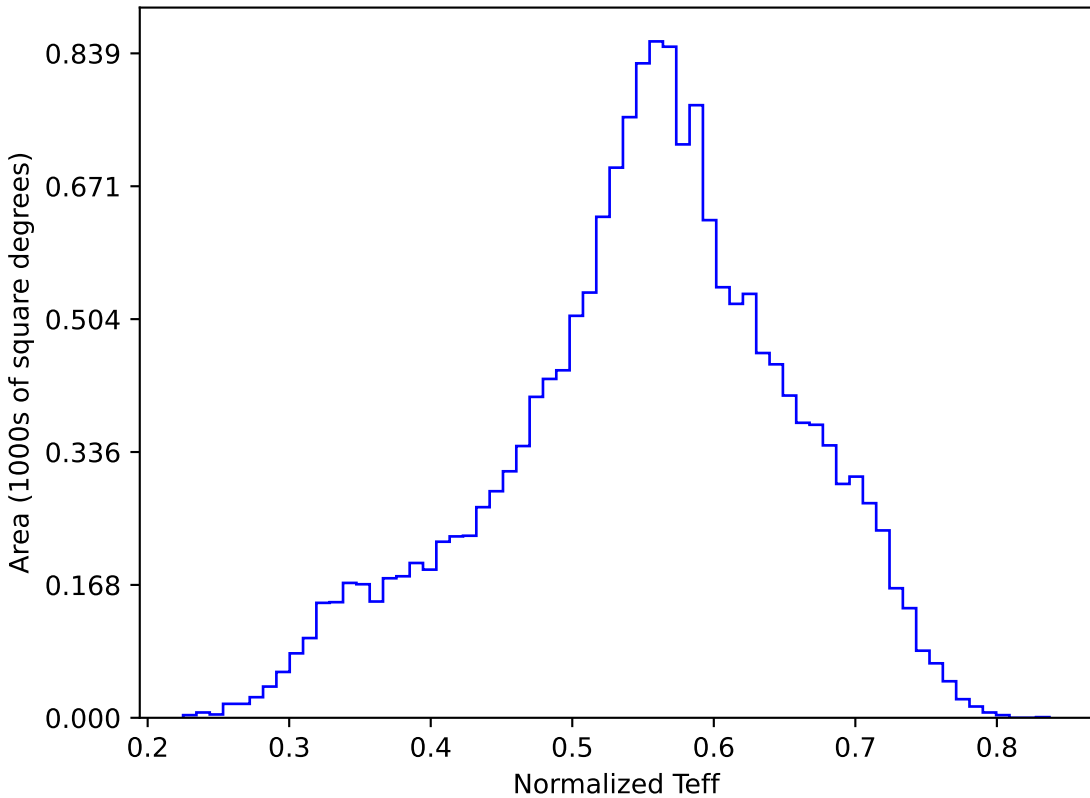
ddf_half_v3.4_10yrs WFD y band: Normalized Teff
