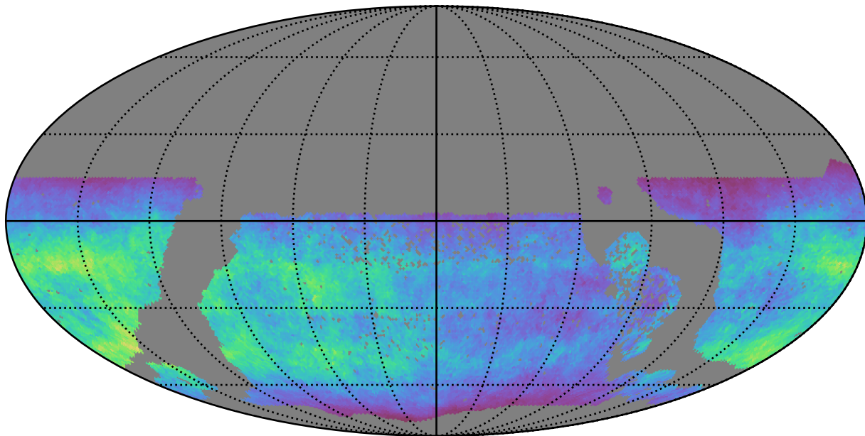
ddf_half_v3.4_10yrs WFD u band: Normalized Teff
