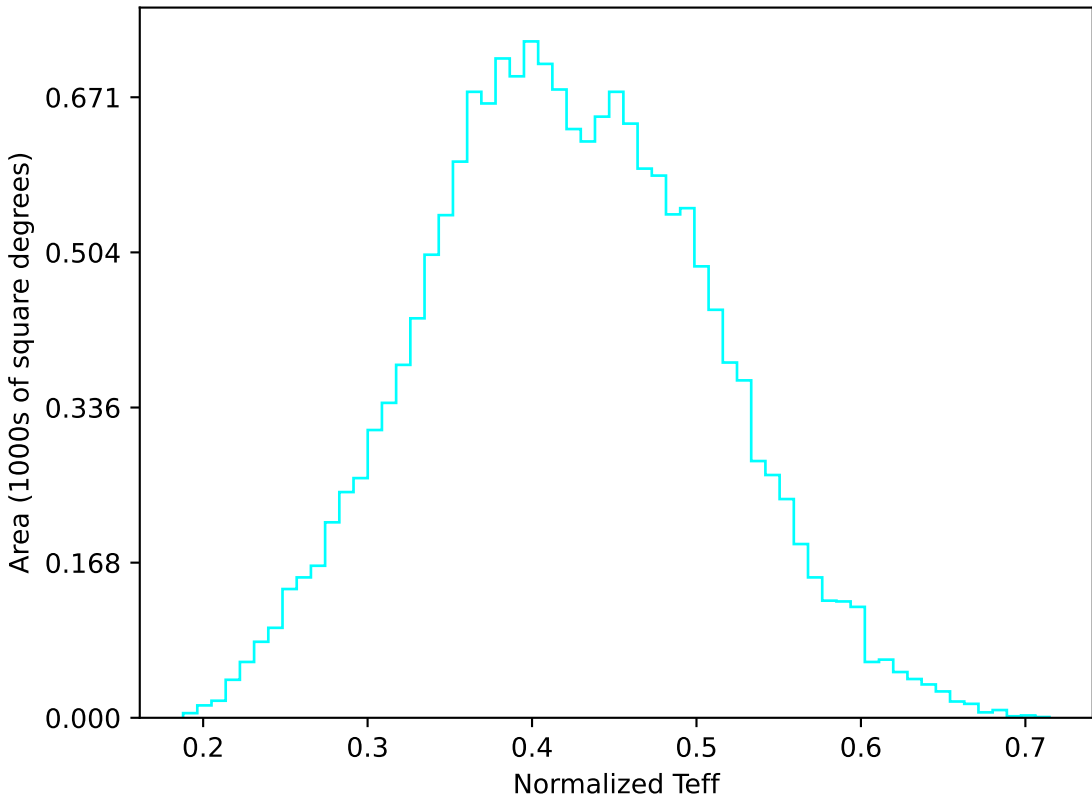
ddf_half_v3.4_10yrs WFD u band: Normalized Teff
