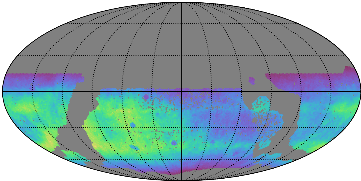
ddf_half_v3.4_10yrs WFD r band: Normalized Teff
