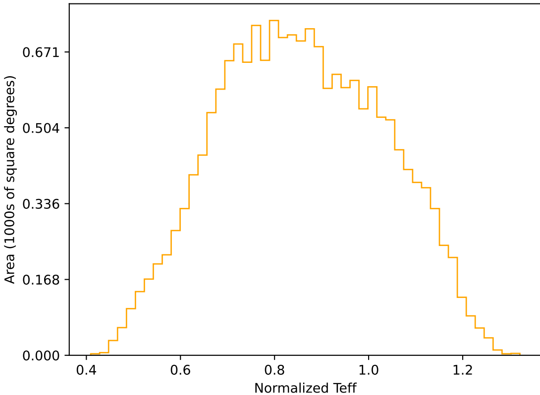
ddf_half_v3.4_10yrs WFD r band: Normalized Teff
