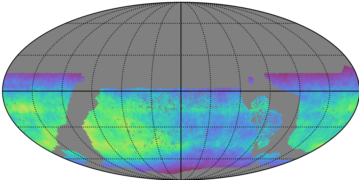
ddf_half_v3.4_10yrs WFD i band: Normalized Teff
