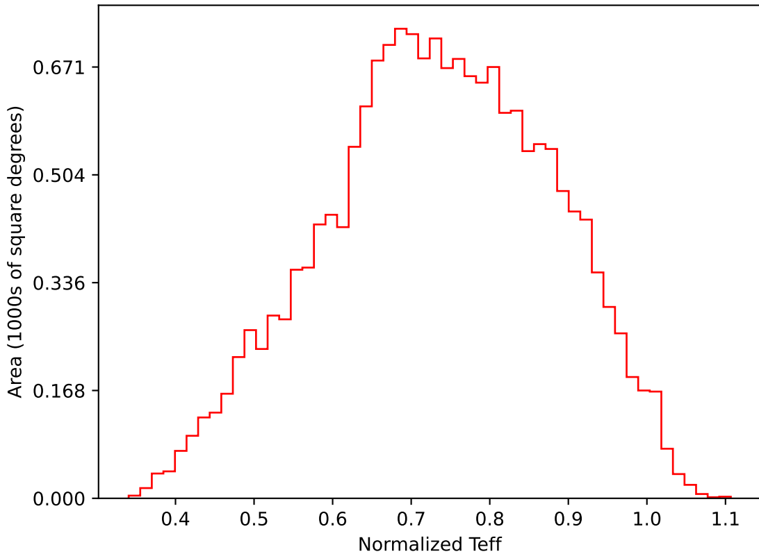
ddf_half_v3.4_10yrs WFD i band: Normalized Teff
