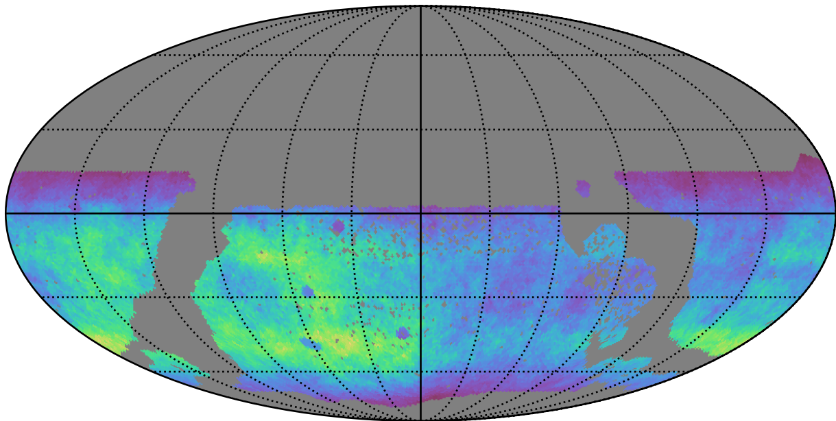
ddf_half_v3.4_10yrs WFD g band: Normalized Teff
